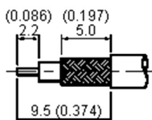
Stripping Dimension
