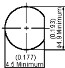
Mounting Hole
