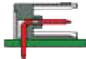
Pitch : 3.5mm (0.138")
