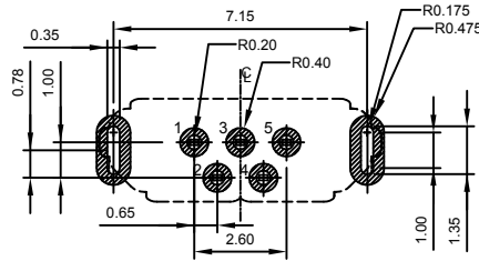
PASTE-IN-HOLE RECOMMENDED P.C.B LAYOUT
