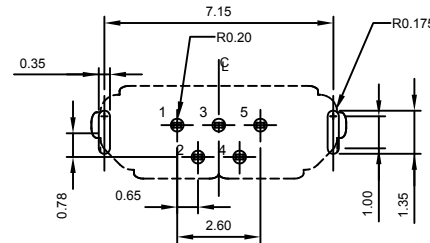
WAVE SOLDER RECOMMENDED P.C.B LAYOUT
