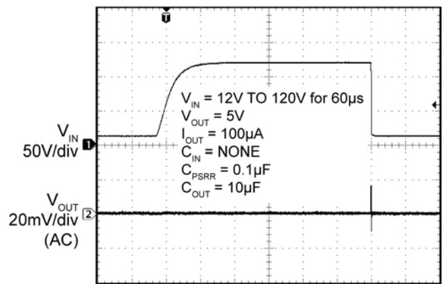
Time (10µs/div)
