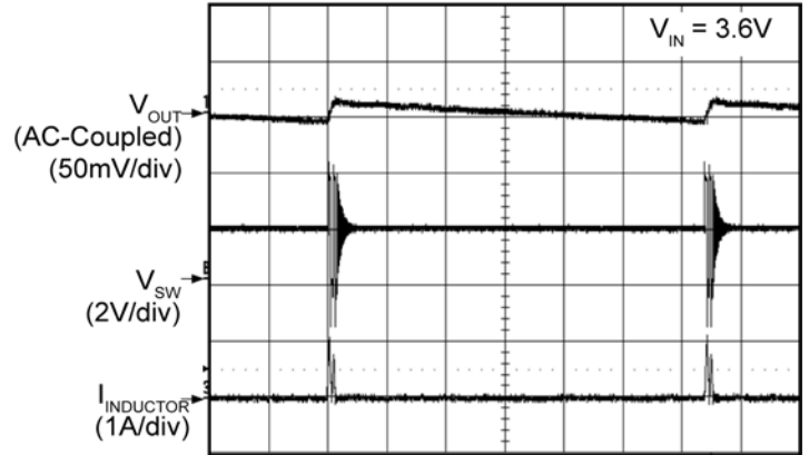
Switching Waveform Discontinuous Mode (10mA)
