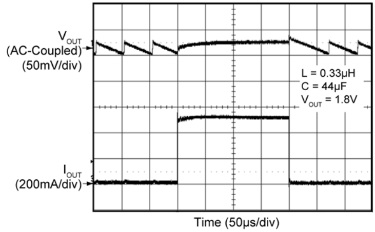
Load Transient (10mA to 500mA)
