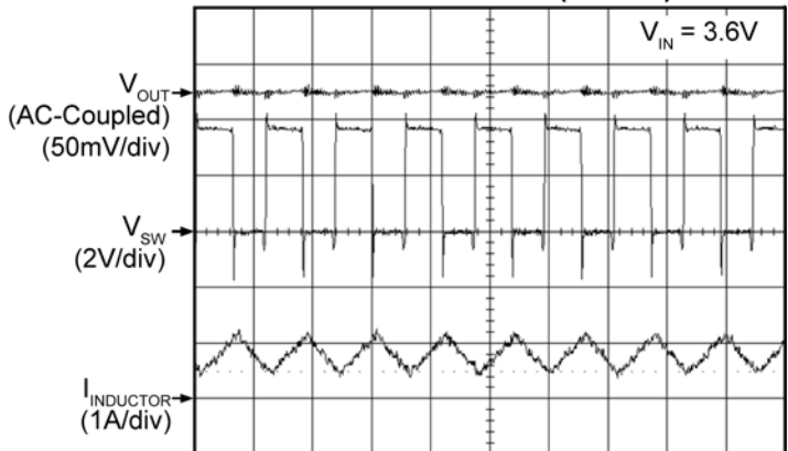
Switching Waveform Continuous Mode (800mA)
