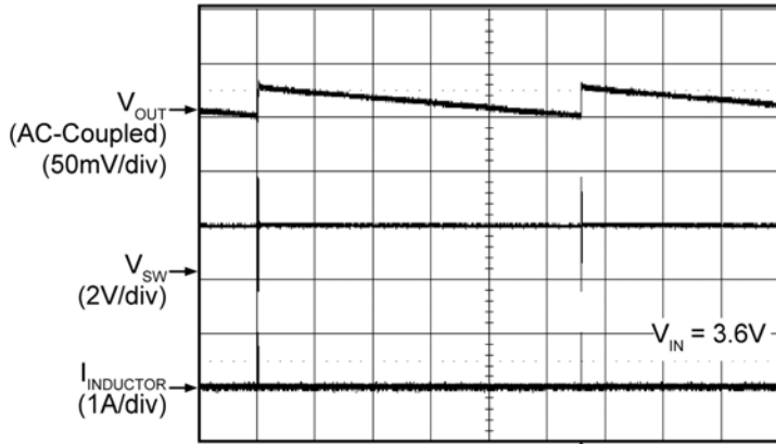
Switching Waveform Discontinuous Mode (1mA)
