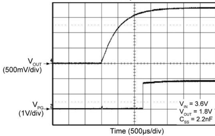
Start-Up PGOOD
