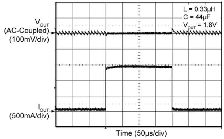
Load Transient (50mA to 1.5A)
