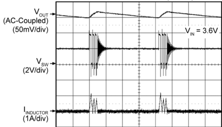
Switching Waveform Discontinuous Mode (50mA)
