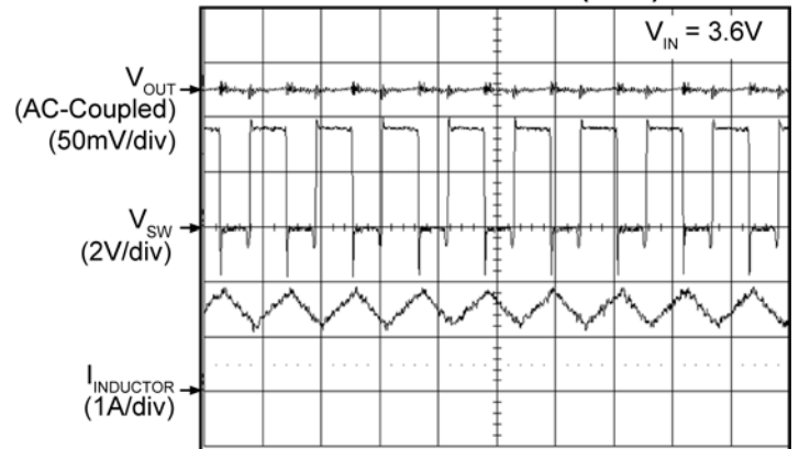
Switching Waveform Continuous Mode (1.5A)
