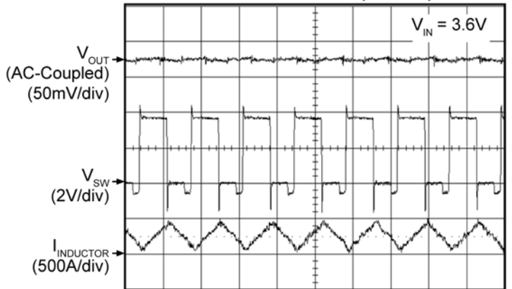
Switching Waveform Continuous Mode (500mA)
