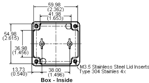
Box - Inside
