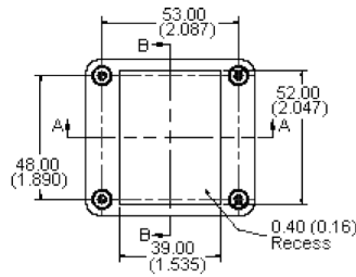
Assembly - Top
