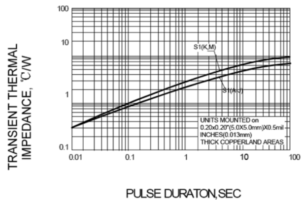
FIG.6-TRANSIENT THERMAL IMPEDANCE
