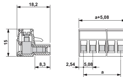
Dimensioned drawing
