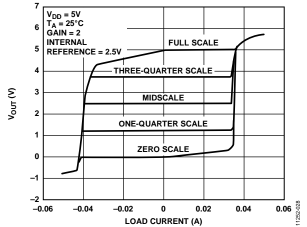
Figure 27. Source and Sink Capability at V_{DD} = 5V
