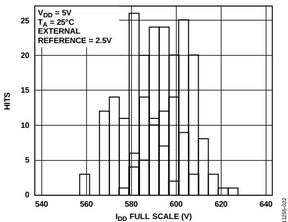
Figure 22. I_{DD} Histogram
