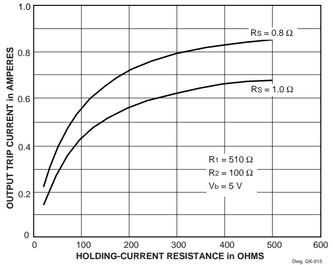
FIGURE 5A. HOLD-CURRENT RESISTANCE (SLA7024M and SMA7029M)
