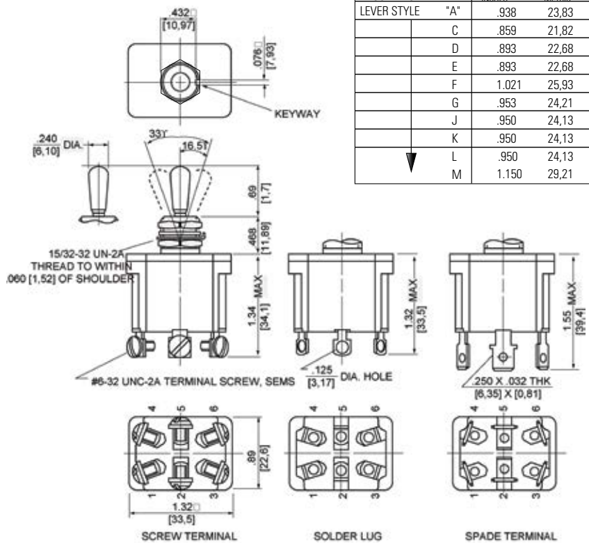
Terminal Identification
