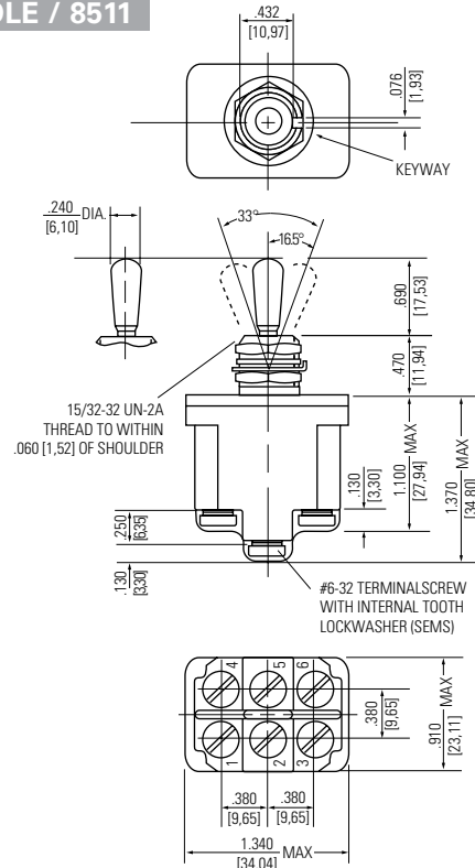
Terminal Identification
