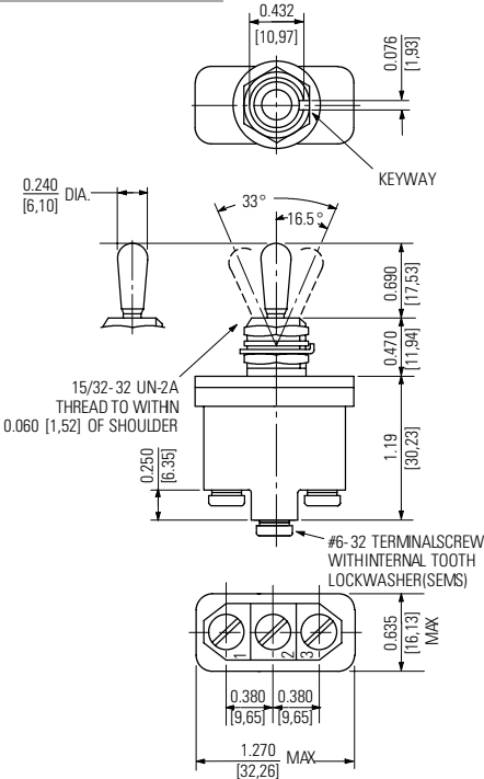
Terminal Identification
