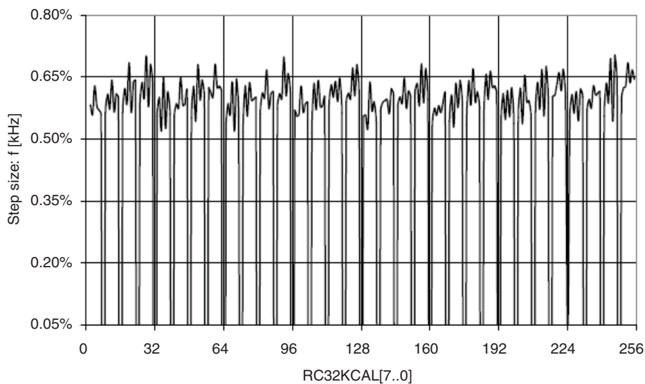
Figure 33-76. Internal 32.768kHz oscillator calibration step size. T = -40 to 85^{\circ}C , V_{CC} = 3V .
