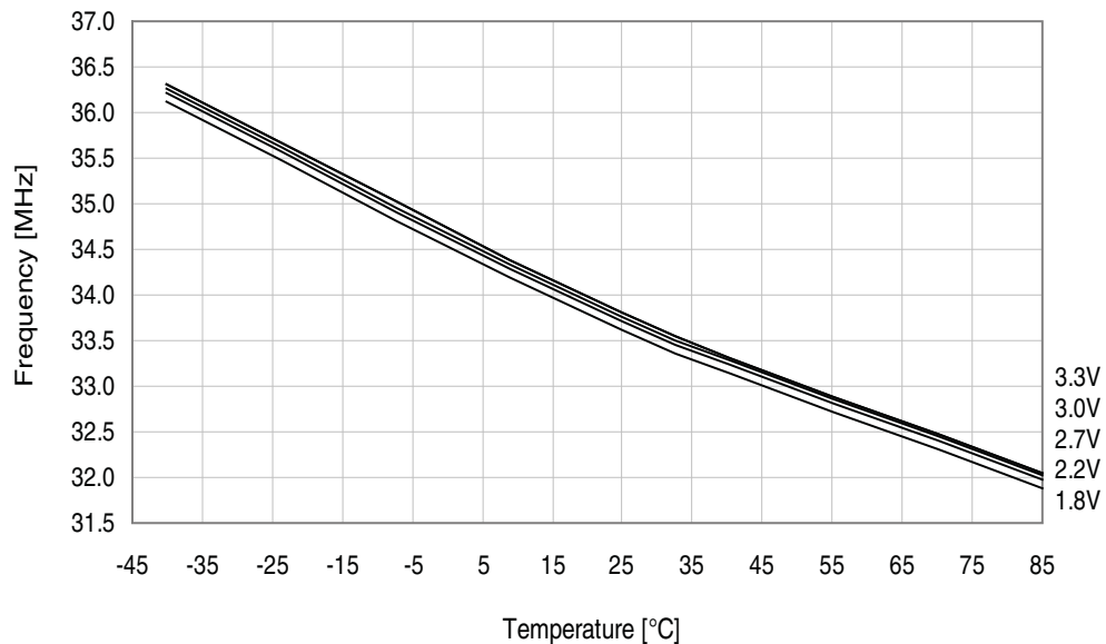
Figure 33-344. 32MHz internal oscillator frequency vs. temperature. DFLL disabled.
