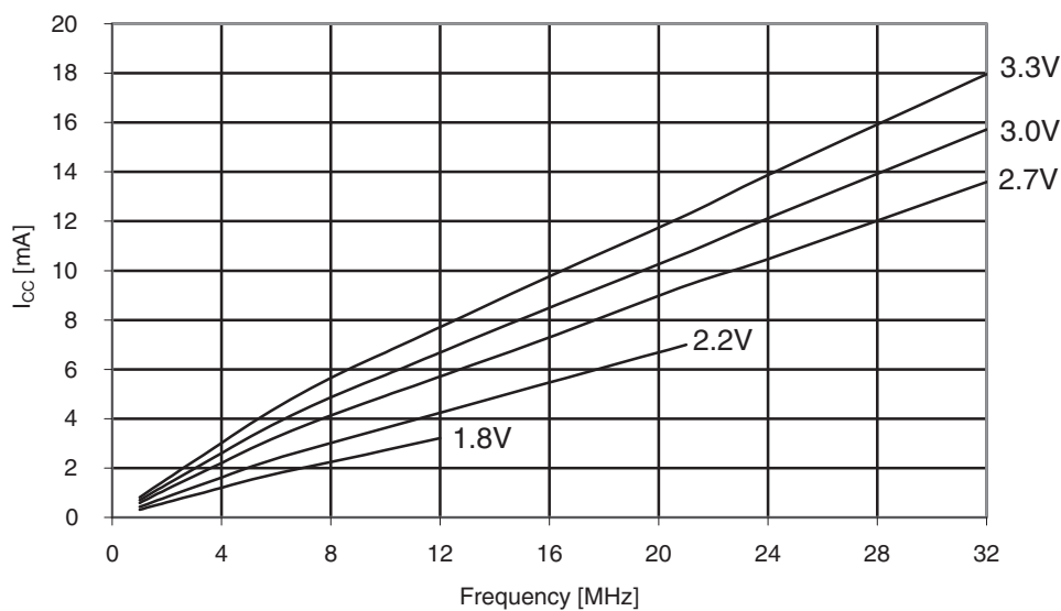
Figure 33-44. Active supply current vs. frequency. f_{\text{SYS}} = 1 - 32\text{MHz} external clock, T = 25^\circ\text{C} .
