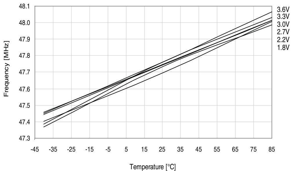
Figure 33-215. 48MHz internal oscillator frequency vs. temperature. DFLL enabled, from the 32.768kHz internal oscillator.
