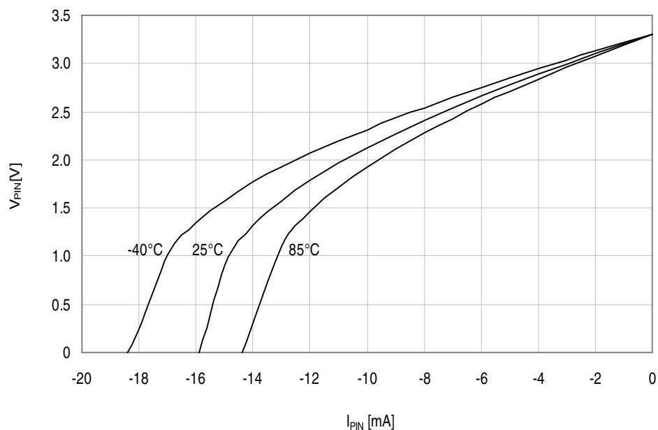
Figure 33-308. I/O pin output voltage vs. source current. V_{CC} = 3.3V .
