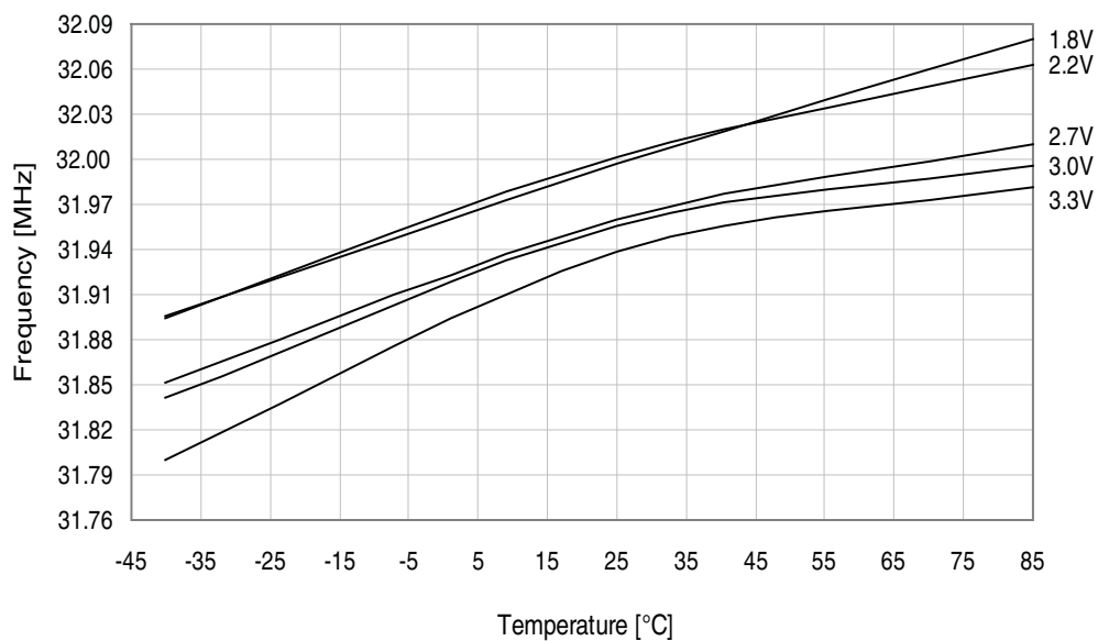
Figure 33-345. 32MHz internal oscillator frequency vs. temperature. DFLL enabled, from the 32.768kHz internal oscillator.
