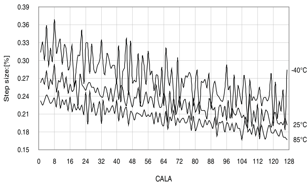
Figure 33-346. 32MHz internal oscillator CALA calibration step size. V_{CC} = 3.0V .
