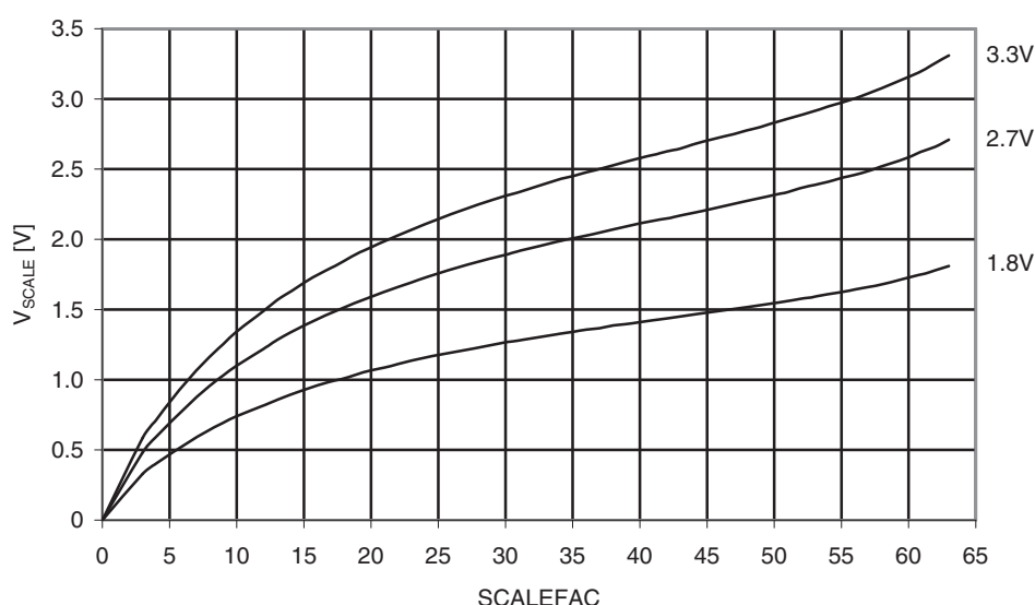
Figure 34-1. Analog comparator voltage scaler vs. scalefac.
