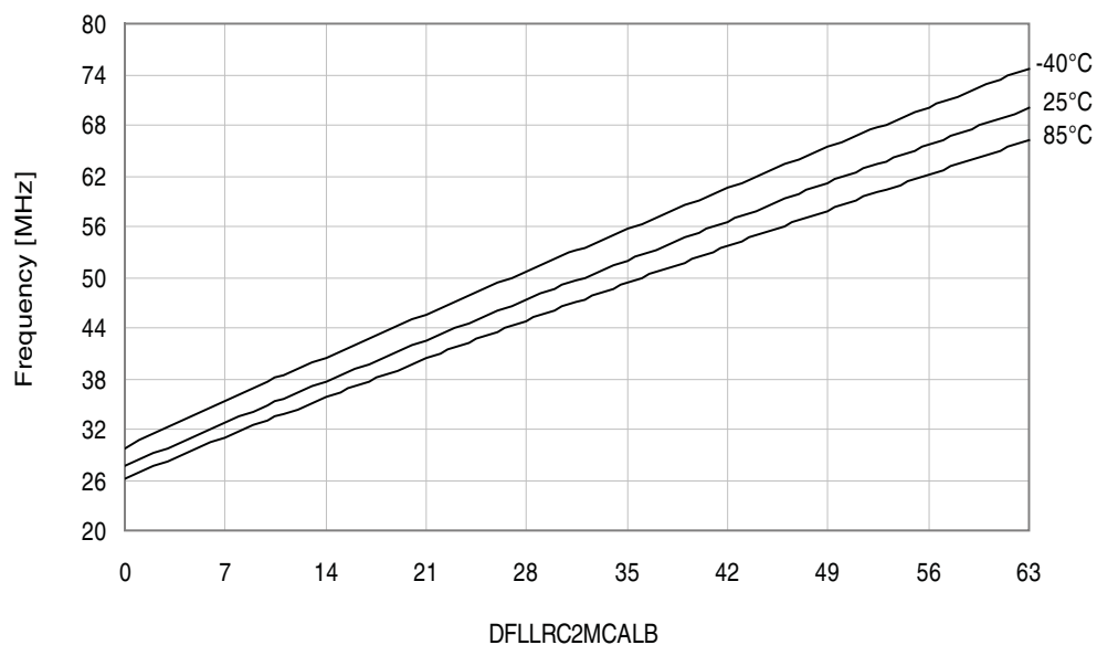
Figure 33-347. 32MHz internal oscillator frequency vs. CALB calibration value. V_{CC} = 3.0V .
