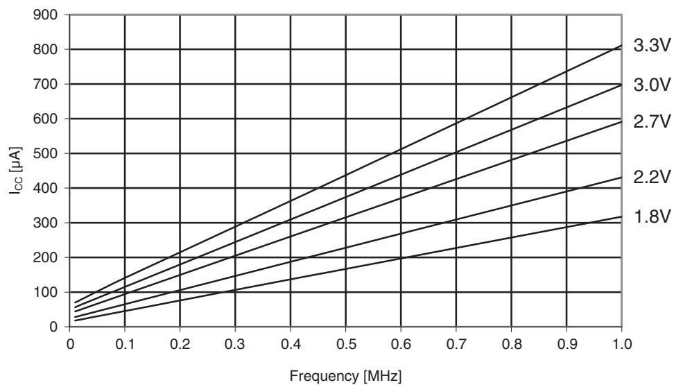
Figure 33-43. Active supply current vs. frequency. f_{\text{SYS}} = 0 - 1\text{MHz} external clock, T = 25^\circ\text{C} .
