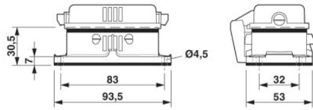
Dimensional drawing
