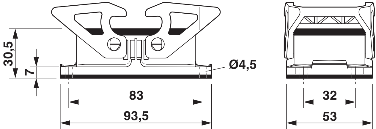
Dimensioned drawing
