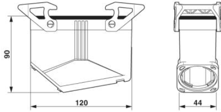
Dimensioned drawing
