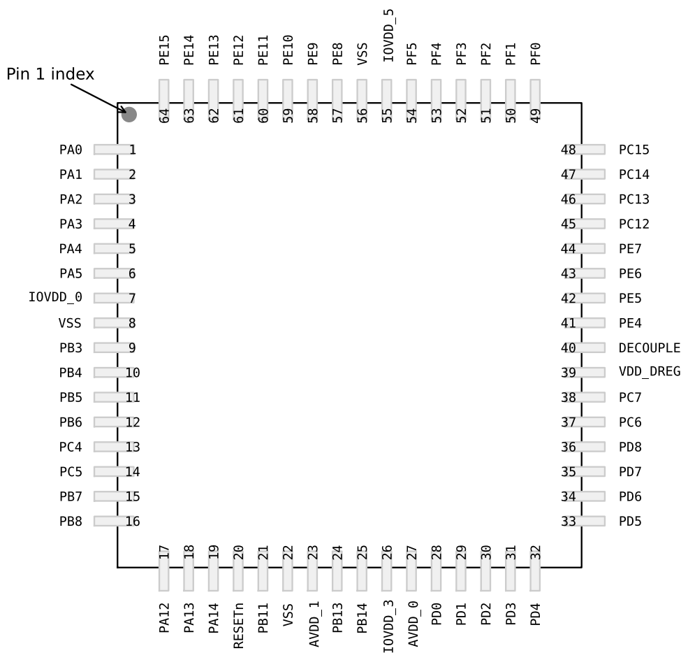
Figure 4.1. EFM32TG842 Pinout (top view, not to scale)
