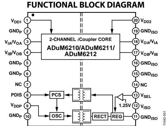
Figure 1. ADuM6210/ADuM6211/ADuM6212
