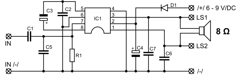
B182 | Amplifier 1 W | 12-0240P
