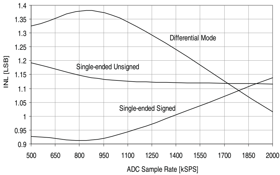
Figure 37-292. INL error vs. sample rate. T = 25°C, V CC = 3.6V, V REF = 3.0V external.
