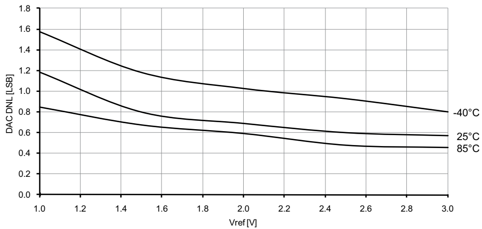
Figure 37-220. DAC DNL error vs. V_{REF} . V_{CC} = 3.6V .
