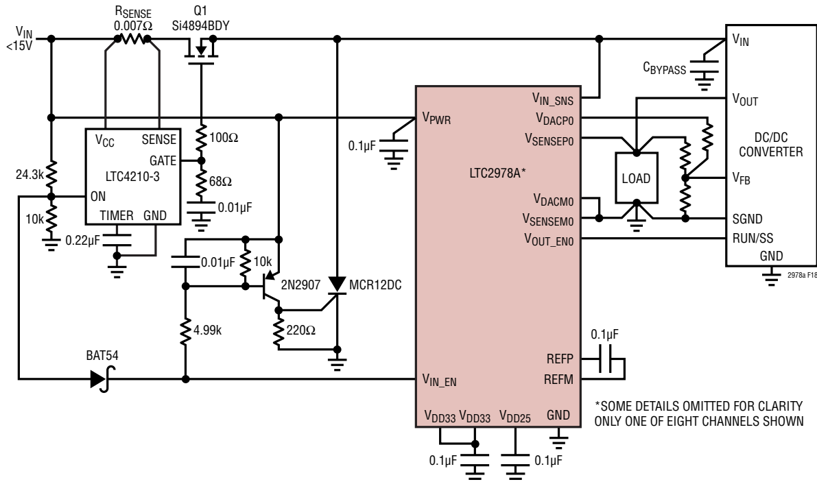
Figure 18. LTC2978A Application Circuit with Crowbar Protection on Intermediate Bus
