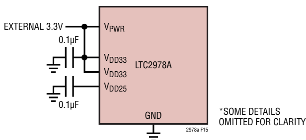
Figure 15. Powering LTC2978A from External 3.3V Supply
