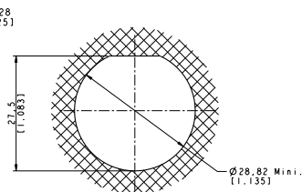
Panel Drilling
