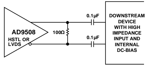
Figure 38. AC-Coupled LVDS or HSTL Output Driver (100 Ω Resistor Can Go on Either Side of Decoupling Capacitors Placed As Close As Possible To The Destination Receiver)
