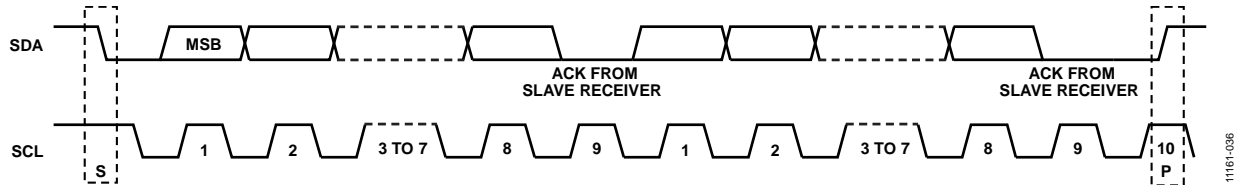
Figure 56. Acknowledge Bit
