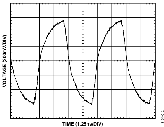
Figure 11. CMOS Output Waveform @ 200 MHz with 10 pF Load
