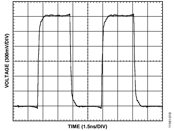
Figure 18. HSTL Differential Output Waveform @ 156.25 MHz
