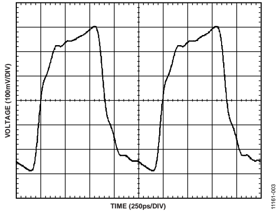
Figure 3. LVDS Differential Output Waveform @ 800 MHz
