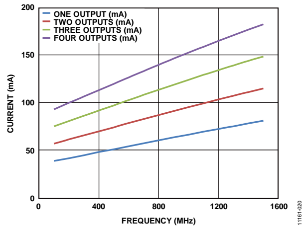
Figure 19. Power Supply Current vs. Frequency and Number of Outputs Used, HSTL
