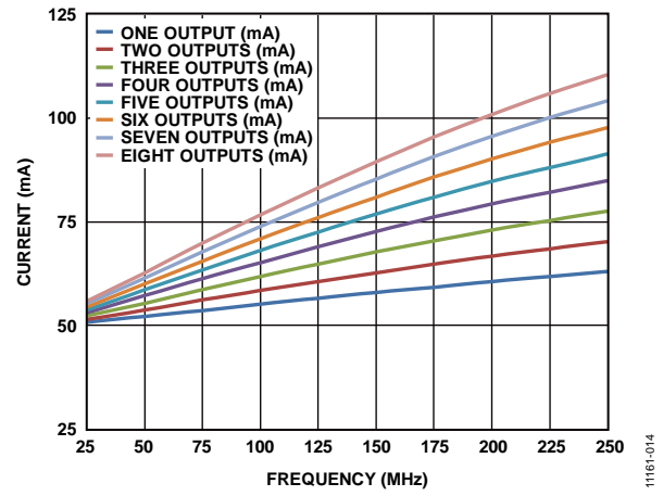
Figure 13. Power Supply Current vs. Frequency vs. Number of Outputs Used, CMOS
