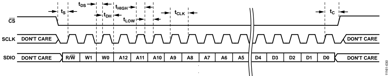
Figure 50. Serial Control Port Write—MSB First, 16-Bit Instruction, Timing Measurements
