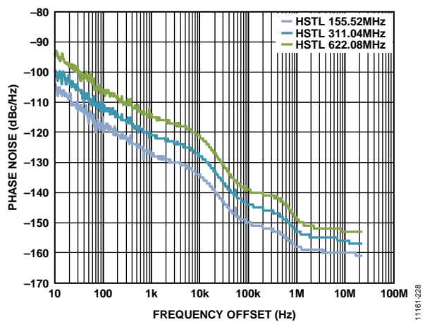
Figure 26. Absolute Phase Noise in HSTL Mode with Clock Input @ 622.08 MHz and Outputs = 622.08 MHz, 311.04 MHz, 155.52 MHz
