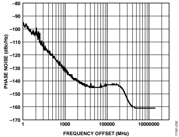
Figure 28. Absolute Phase Noise of Clock Source @ 622.08 MHz
