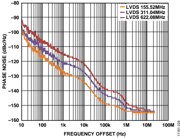
Figure 27. Absolute Phase Noise in LVDS Mode with Clock Input @ 622.08 MHz and Outputs = 622.08 MHz, 311.04 MHz, 155.52 MHz
