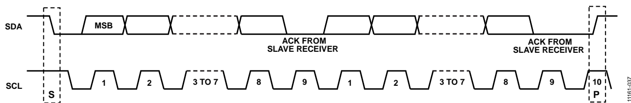
Figure 57. Data Transfer Process (Master Write Mode, Two-Byte Transfer)
