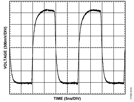
Figure 12. CMOS Output Waveform @ 50 MHz with 10 pF Load
