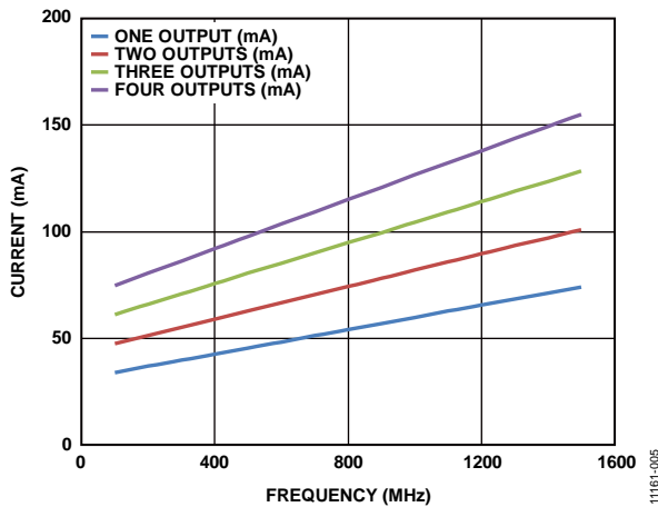
Figure 5. Power Supply Current vs. Frequency and Number of Outputs Used, LVDS
