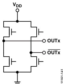
Figure 43. LVDS/HSTL Output Simplified Equivalent Circuit
