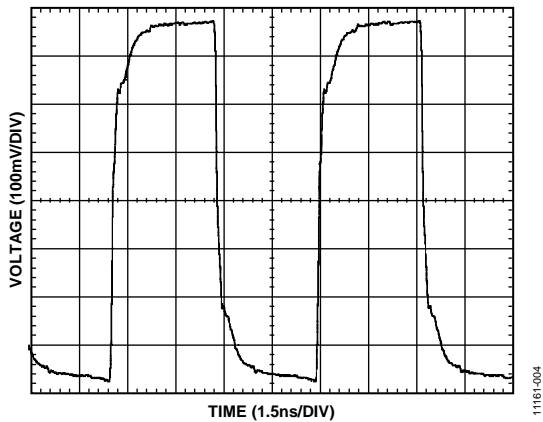
Figure 4. LVDS Differential Output Waveform @ 156.25 MHz
