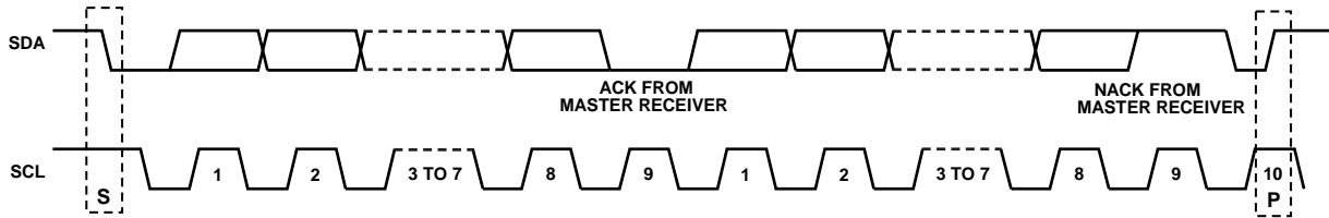
Figure 58. Data Transfer Process (Master Read Mode, Two-Byte Transfer)
