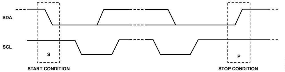
Figure 55. Start and Stop Conditions
