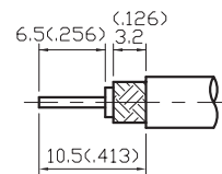
STRIPPING DIMENSION
