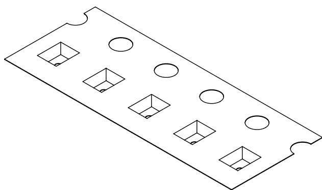
Figure I8. Emitter pocket tape packaging for LUXEON Z.
