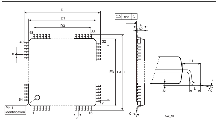
Figure 39. LQFP64 – 10 x 10 mm, 64 pin low-profile quad flat package outline (1)
