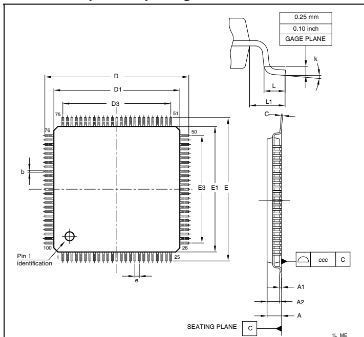
Figure 37. LQFP100, 14 x 14 mm, 100-pin low-profile quad flat package outline (1)
