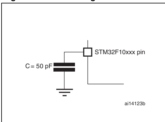
Figure 8. Pin loading conditions
