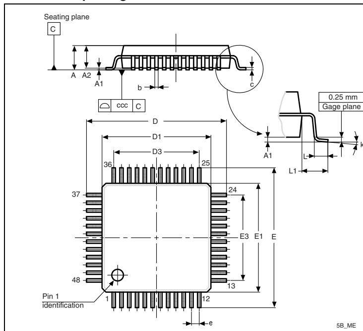
Figure 43. LQFP48 – 7 x 7 mm, 48-pin low-profile quad flat package outline (1)
