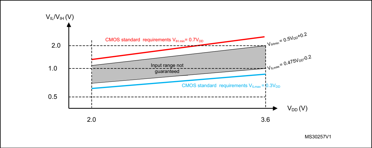
Figure 18. Five volt tolerant (FT and FTf) I/O input characteristics - CMOS port
