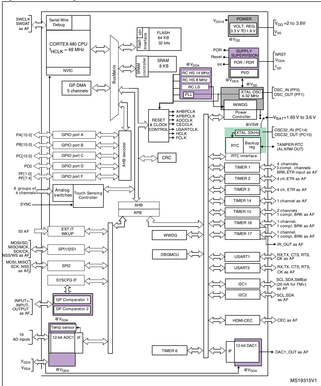
Figure 1. Block diagram
