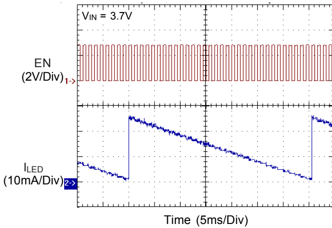
Pulse Dimming Operation
