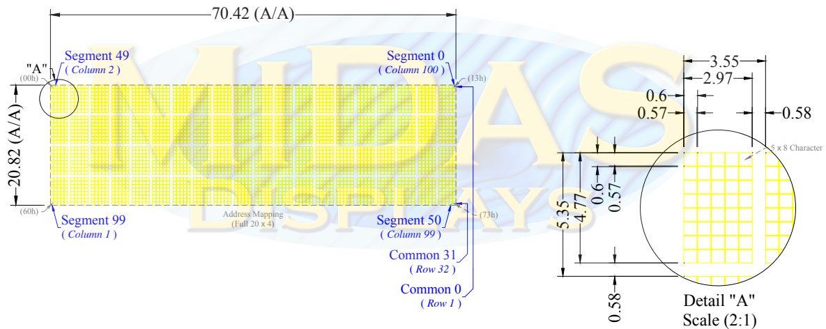
Address Mapping
