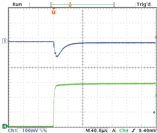
Step Load Transient Response (Vin=12V, Vout=1.8V, Cload=12x10µF X5R 0805 ceramic, total 120µF, Iout=0A to 3A) Top trace=Vout, Bottom trace=Iout
