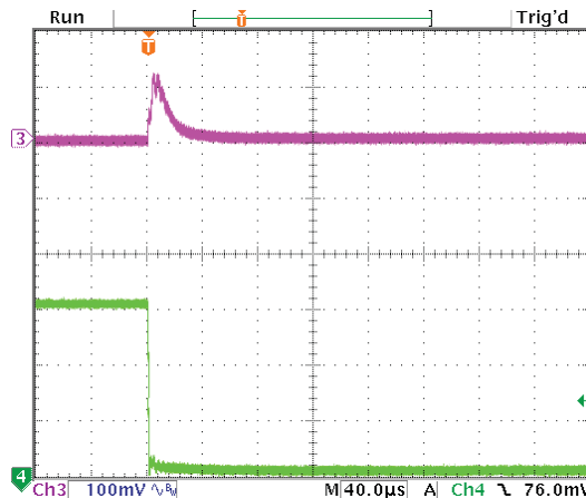
Step Load Transient Response (Vin=4.5V, Vout=1.8V, Cload=5x10µF X5R 0805 ceramic, total 50µF, Iout=3A to 0A) Top trace=Vout, Bottom trace=Iout
