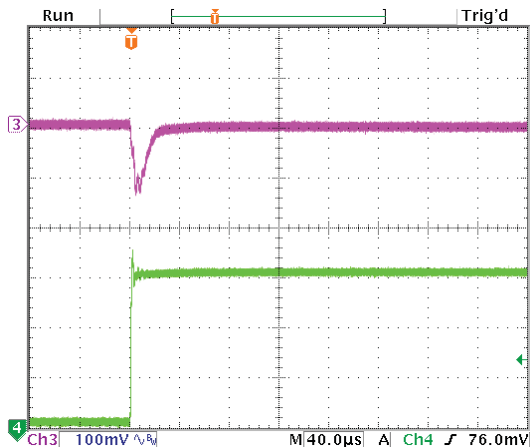
Step Load Transient Response (Vin=4.5V, Vout=1.8V, Cload=5x10µF X5R 0805 ceramic, total 50µF, Iout=0A to 3A) Top trace=Vout, Bottom trace=Iout
