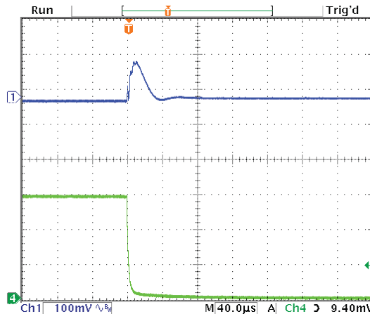
Step Load Transient Response (Vin=12V, Vout=1.8V, Cload=12x10µF X5R 0805 ceramic, total 120µF, Iout=3A to 0A) Top trace=Vout, Bottom trace=Iout
