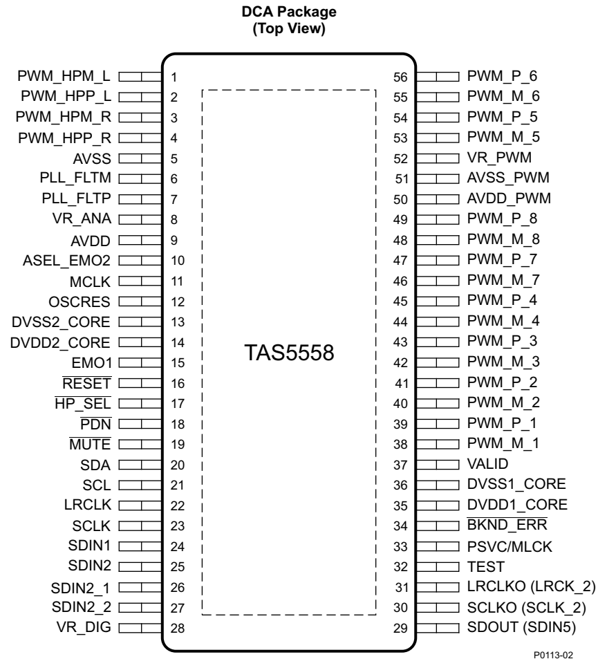
Figure 2-1. TAS5558 Pinout
