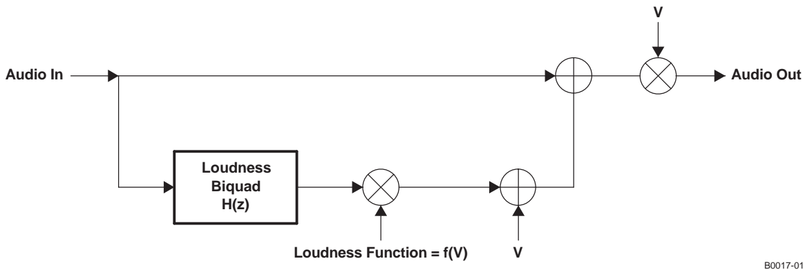
Figure 3-13. Loudness Compensation Functional Block Diagram
