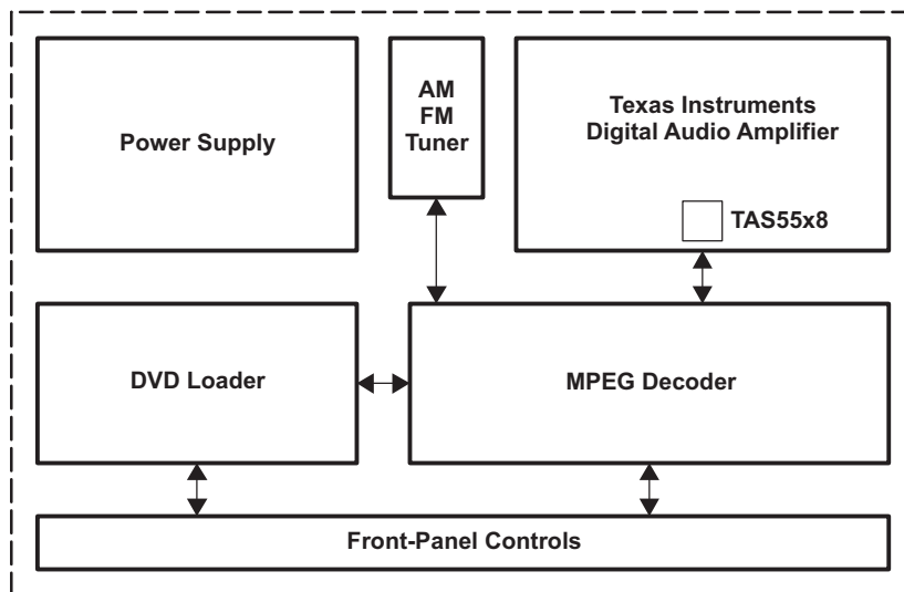
Figure 9-1. Typical TAS5558 Application (DVD Receiver)
