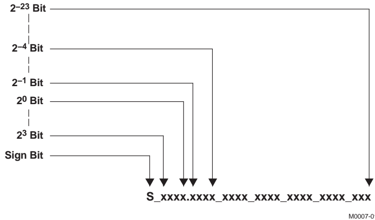
Figure 3-7. 5.23 Format
