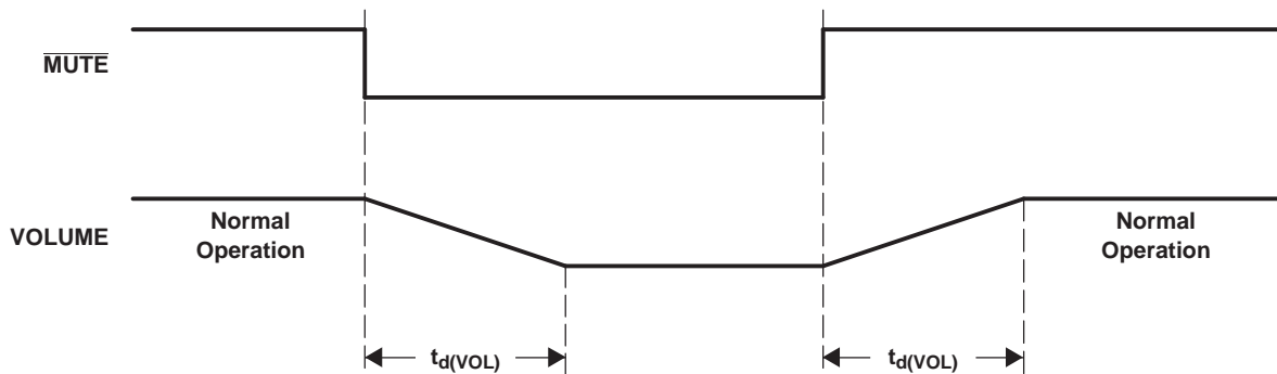
Figure 7-7. Mute Timing
