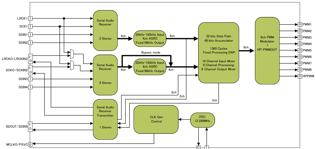
Figure 9-3. Digital Audio Signal Flow Block Diagram
