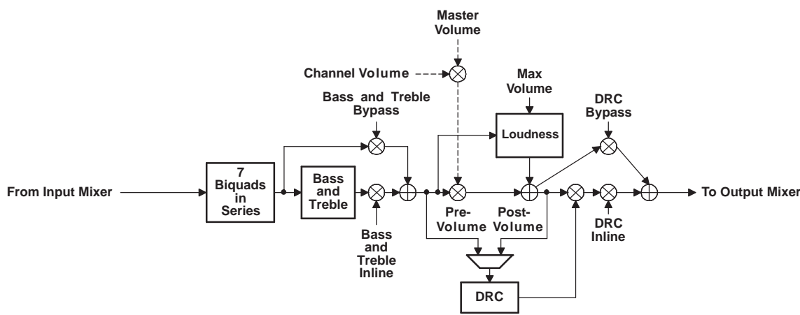
Figure 3-15. DRC Positioning in TAS5558 Processing Flow
