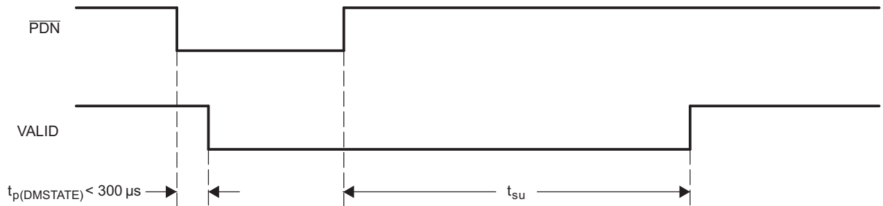
Figure 7-5. Power-Down Timing
