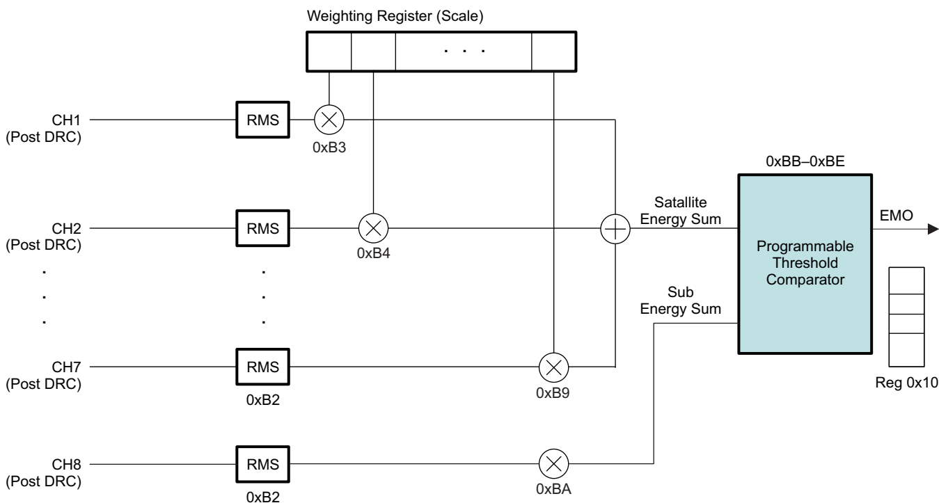
Figure 6-1. Energy Manager
