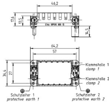
Drawing Dimensions in mm (Inch) 26.06.2013
