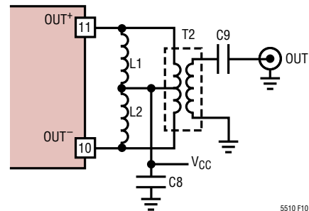
Figure 10. HF Board Output Schematic
