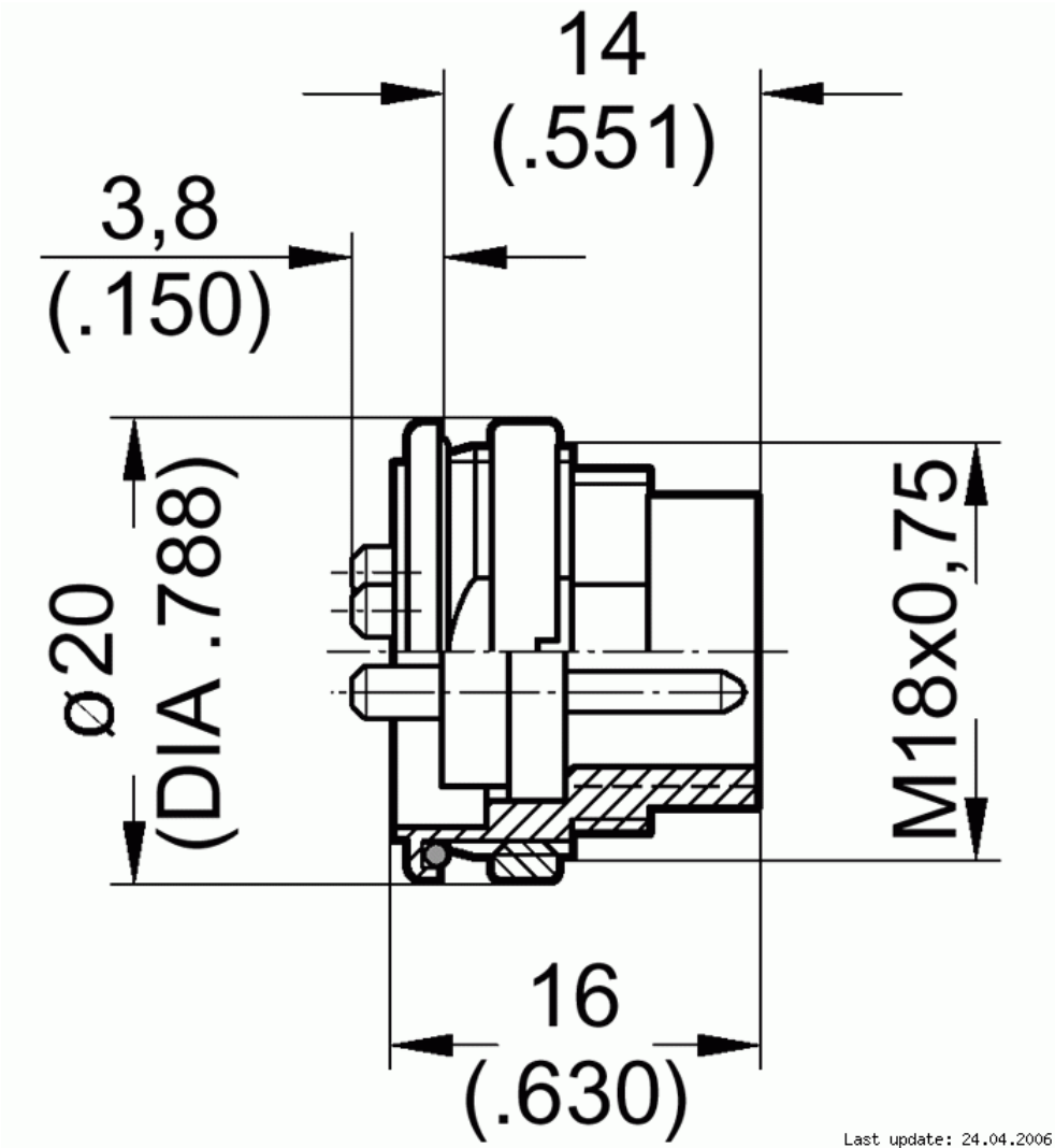
Drawing Dimensions in mm (Inch)
