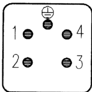
Contact arrangement
