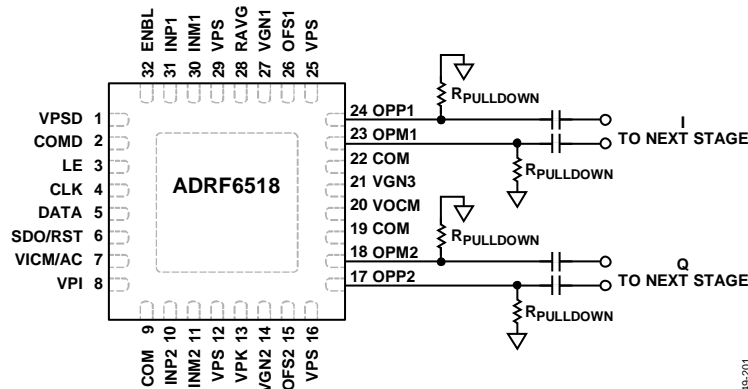
Figure 85. Pull-Down Resistors
