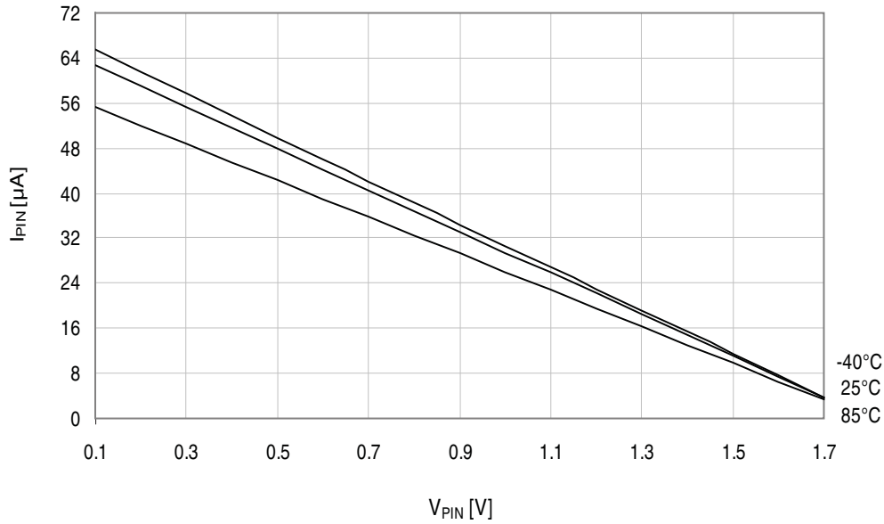
Figure 34-22. I/O pin pull-up resistor current vs. input voltage.
