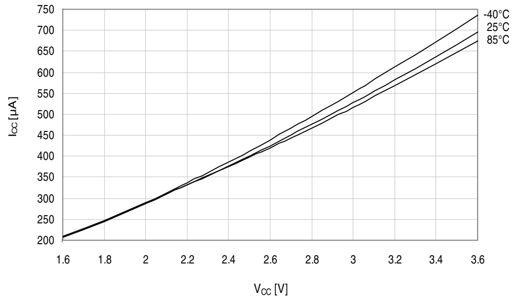
Figure 34-274. Active mode supply current vs. V_{CC} .
