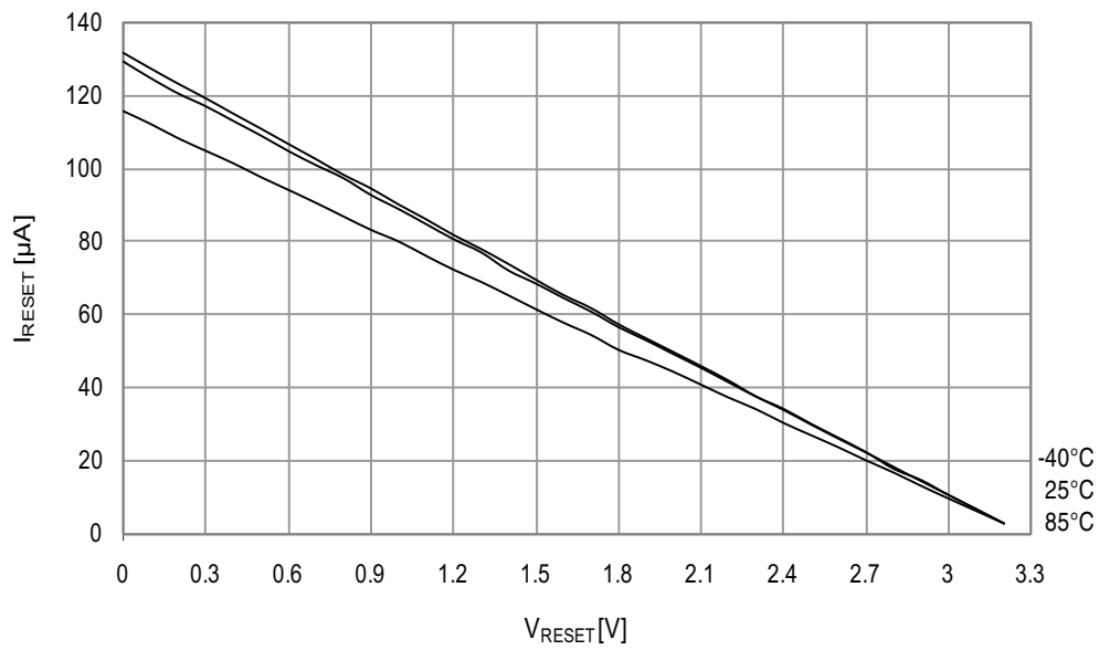
Figure 34-120. Reset pin pull-up resistor current vs. reset pin voltage.
