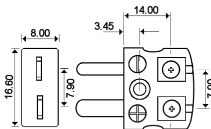
Quick-Wire Miniature Plug
