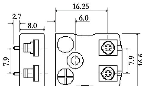
FAR055/0613 JIS Miniature Thermocouple PCB Mounting Socket
