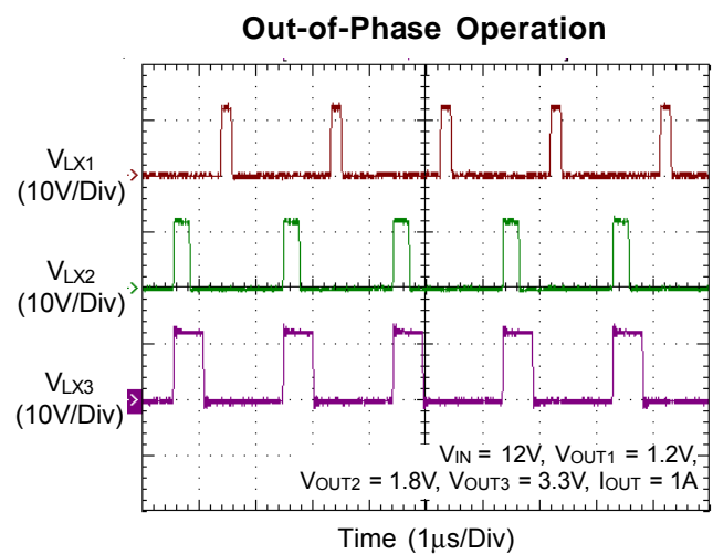
Figure 2. Switching Signals for Each Channel
