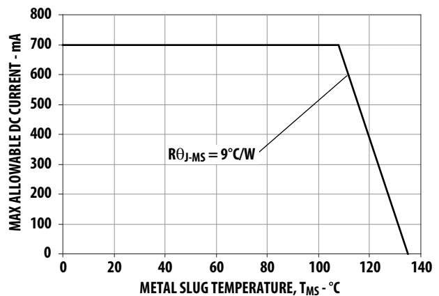
Figure 23. Maximum Forward Current vs. Metal Slug Temperature. Derated based on T_{JMAX} = 135^\circ\text{C} , R_{\theta MS} = 9^\circ\text{C/W}
