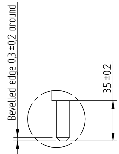
DETAIL A (5:1)
