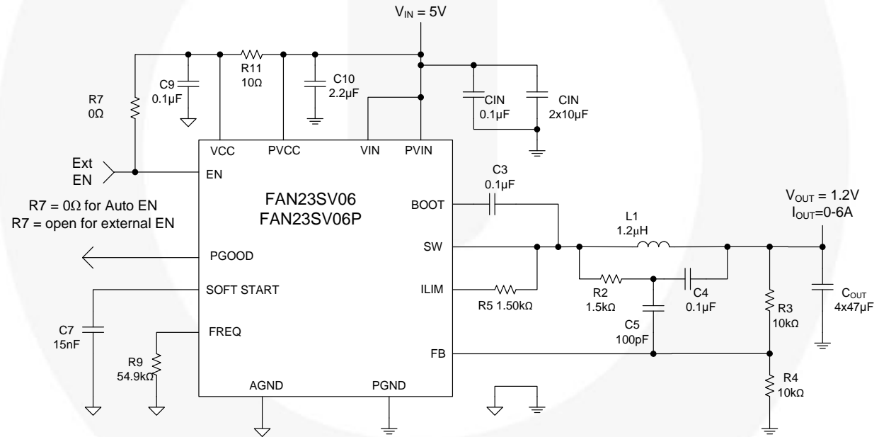
Figure 2. Typical Application with V_{IN} = 5\text{ V}
