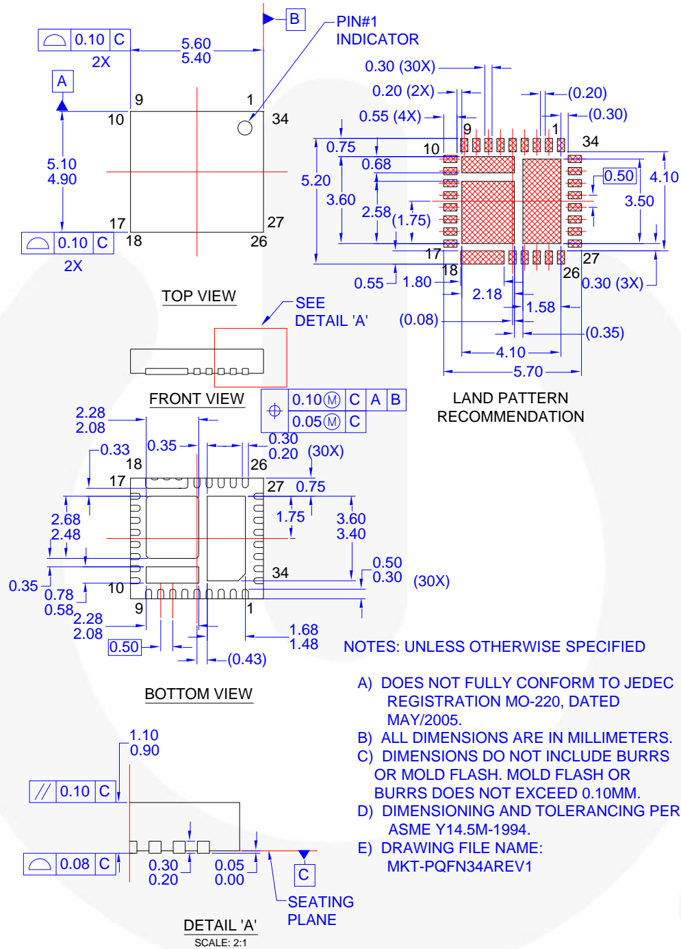
Figure 34.34-Lead, PQFN, 5.5 mm x 5.0 mm Package
