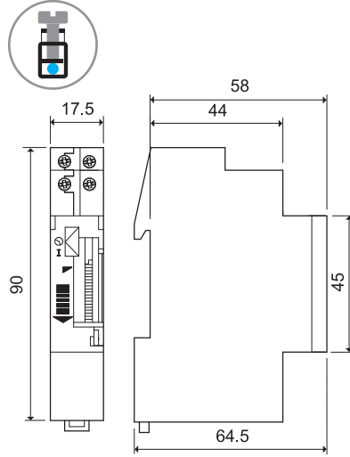
12.11 Screw terminal
