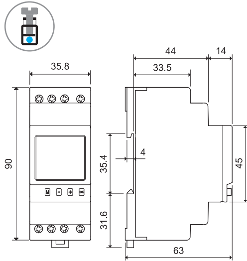
12.51/12.81 Screw terminal
