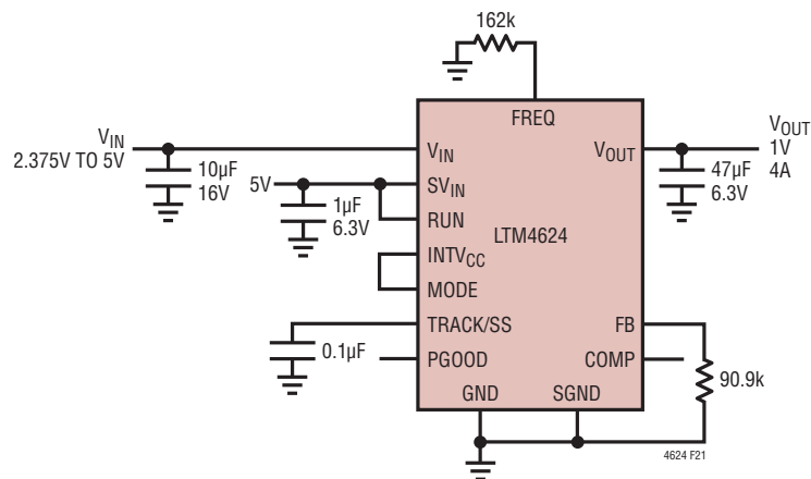
Figure 21. 2.375V_{IN} to 5V_{IN} , 1V Output with 2MHz Operating Frequency
