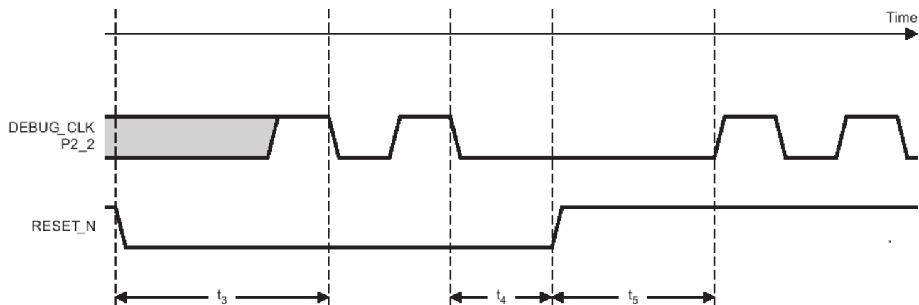
Figure 6 Slave Timing
