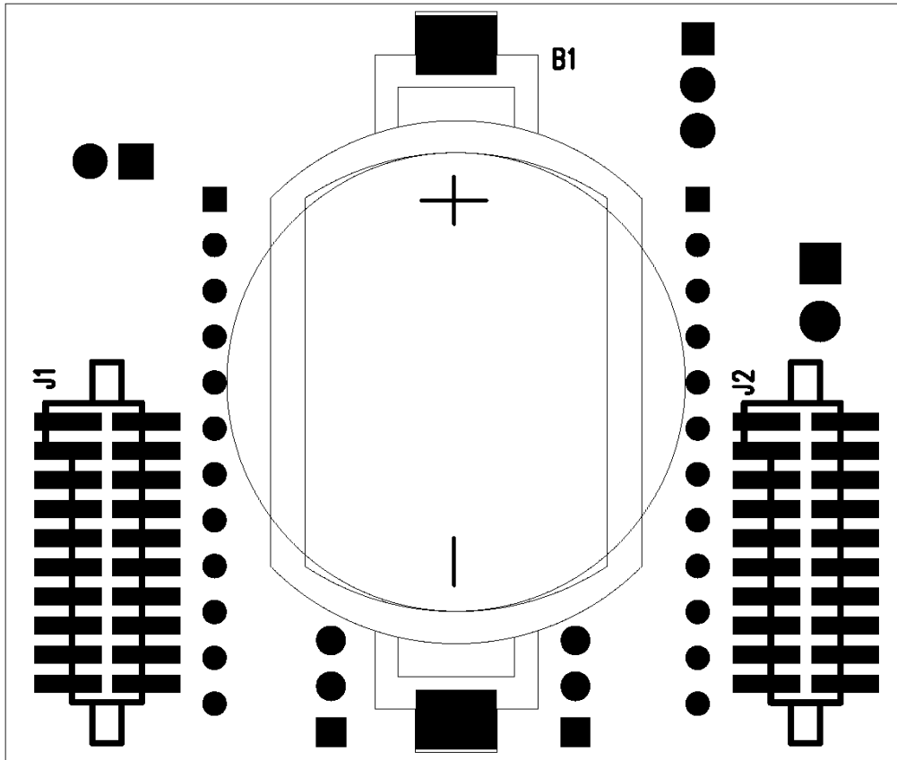
Figure 2 TiWi-uB1 EM Board Bottom
