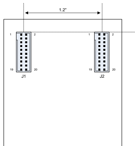
Figure 3 TiWi-uB1 EM Board Bottom
