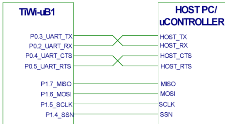
Figure 4 TiWi-uB1 EM Board Interface to Host
