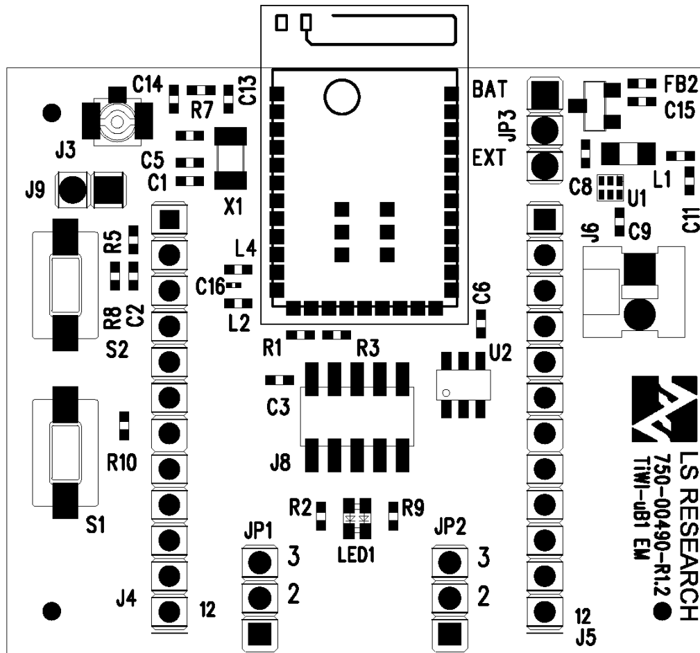
Figure 1 TiWi-uB1 EM Board Top Side
