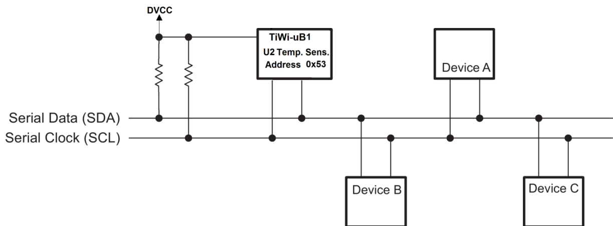
Figure 5 I 2 C Interface TiWi-uB1 EM Board Schematic
