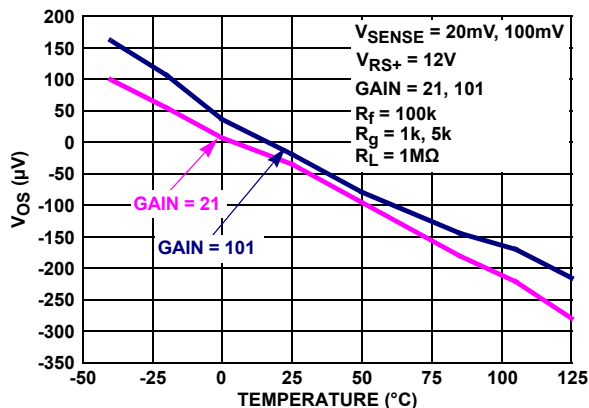
FIGURE 60. V_{OS} ( \mu V ) vs TEMPERATURE
