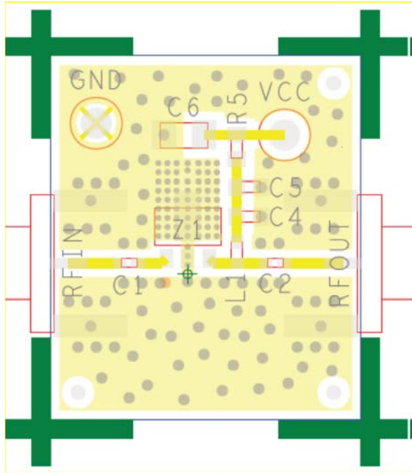
Figure 30. Evaluation Board Layout (Top)
