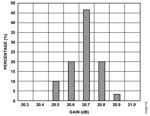
Figure 19. Gain Distribution at 2600 MHz
