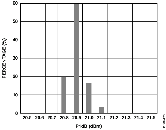
Figure 21. P1dB Distribution at 900 MHz
