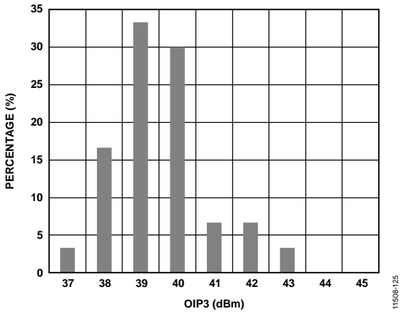
Figure 22. OIP3 Distribution at 900 MHz, P OUT = 0 dBm per Tone
