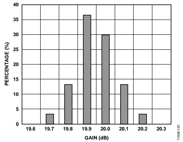
Figure 20. Gain Distribution at 4000 MHz
