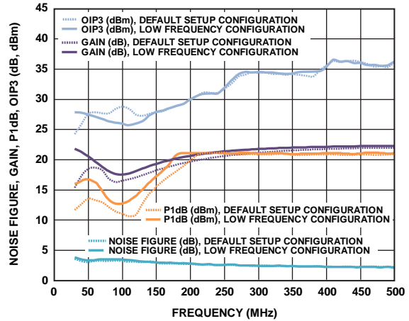
Figure 26. Noise Figure, Gain, P1dB, and OIP3 vs. Frequency, 30 MHz to 500 MHz, Comparison of Performance with the Optimized Settings and the Default Configuration
