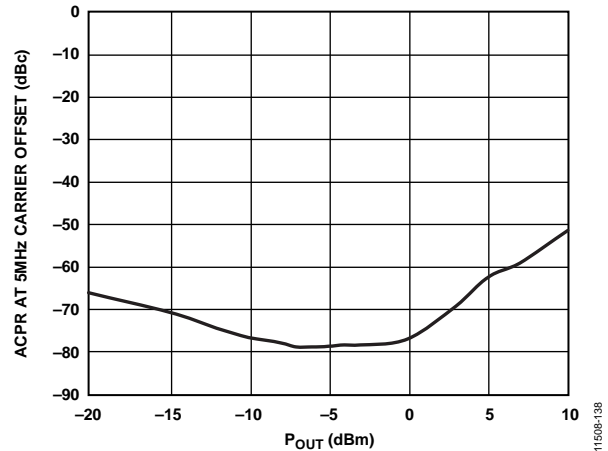
Figure 29. ACPR vs. P_{OUT} , Single W-CDMA Carrier (Test Model 1-64) at 2140 MHz
