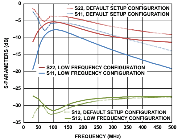
Figure 27. Output Return Loss (S22), Input Return Loss (S11), and Reverse Isolation (S12), 30 MHz to 500 MHz, Comparison of Performance with the Optimized Settings and the Default Configuration
