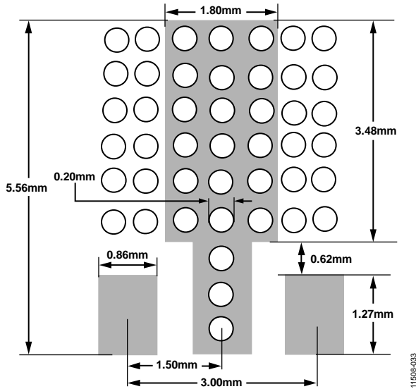
Figure 28. Recommended Land Pattern
