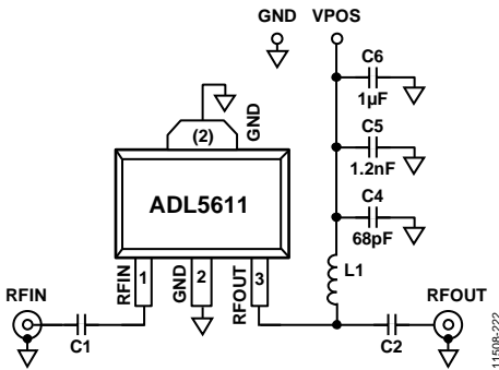
Figure 25. Basic Connections
