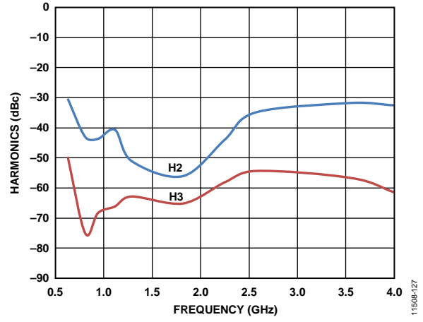
Figure 24. Single-Tone Harmonics vs. Frequency, P OUT = 0 dBm
