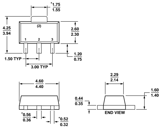
Figure 32. 3-Lead Small Outline Transistor Package [SOT-89] (RK-3)
