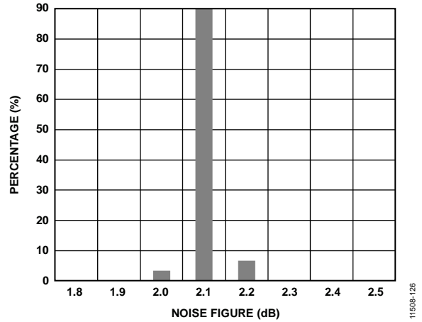
Figure 23. Noise Figure Distribution at 900 MHz
