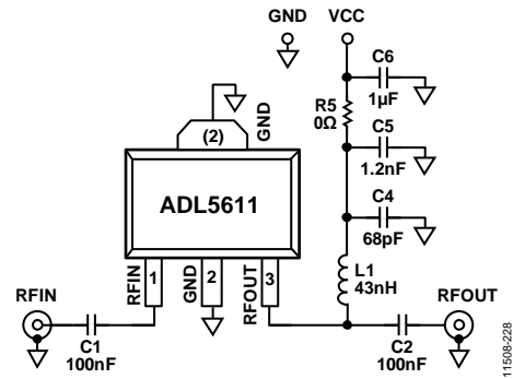
Figure 31. Evaluation Board Schematic
